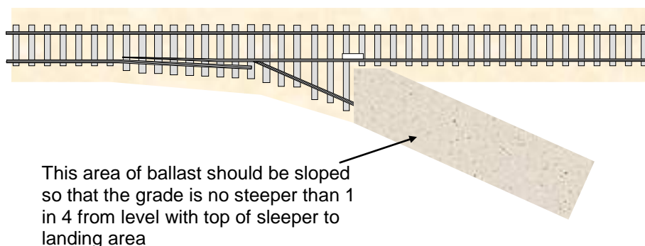
Figure 2 – Ramp to landing zone
