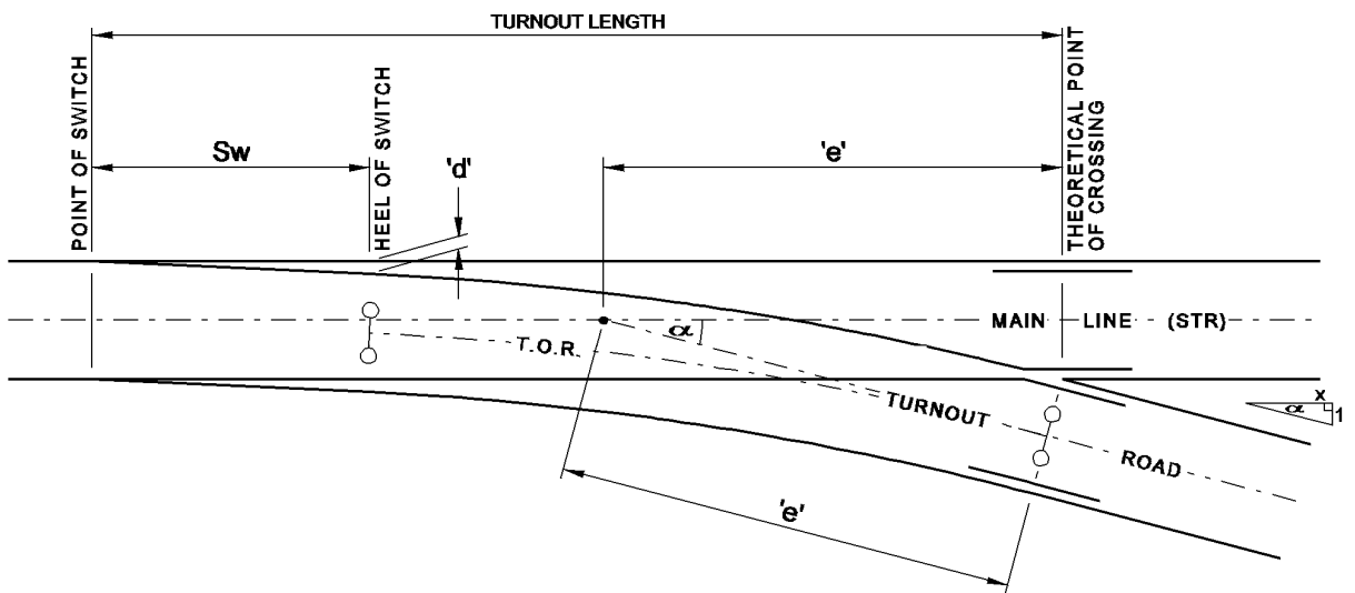
Figure 9 - Curved Crossing Conventional Turnout – short leg curved (drawn for RH turnout)
