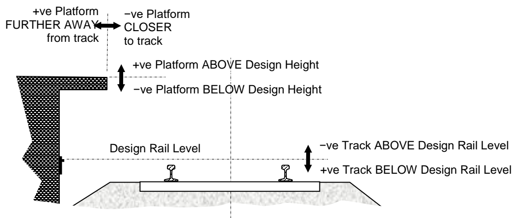
Figure 7 – Measurement Conventions
