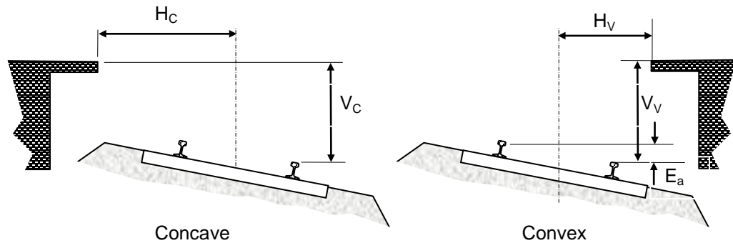
Figure 5 - Platform clearances on curved track
