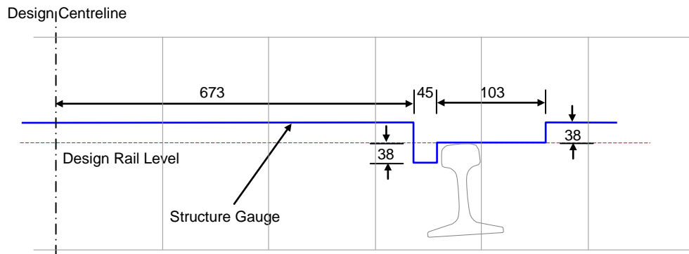
Figure 2 – Structure Gauge Detail at Rail Level
