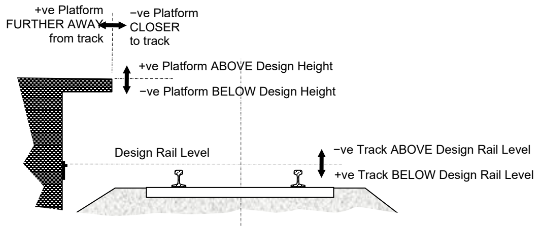
Figure 7 – Measurement Conventions
